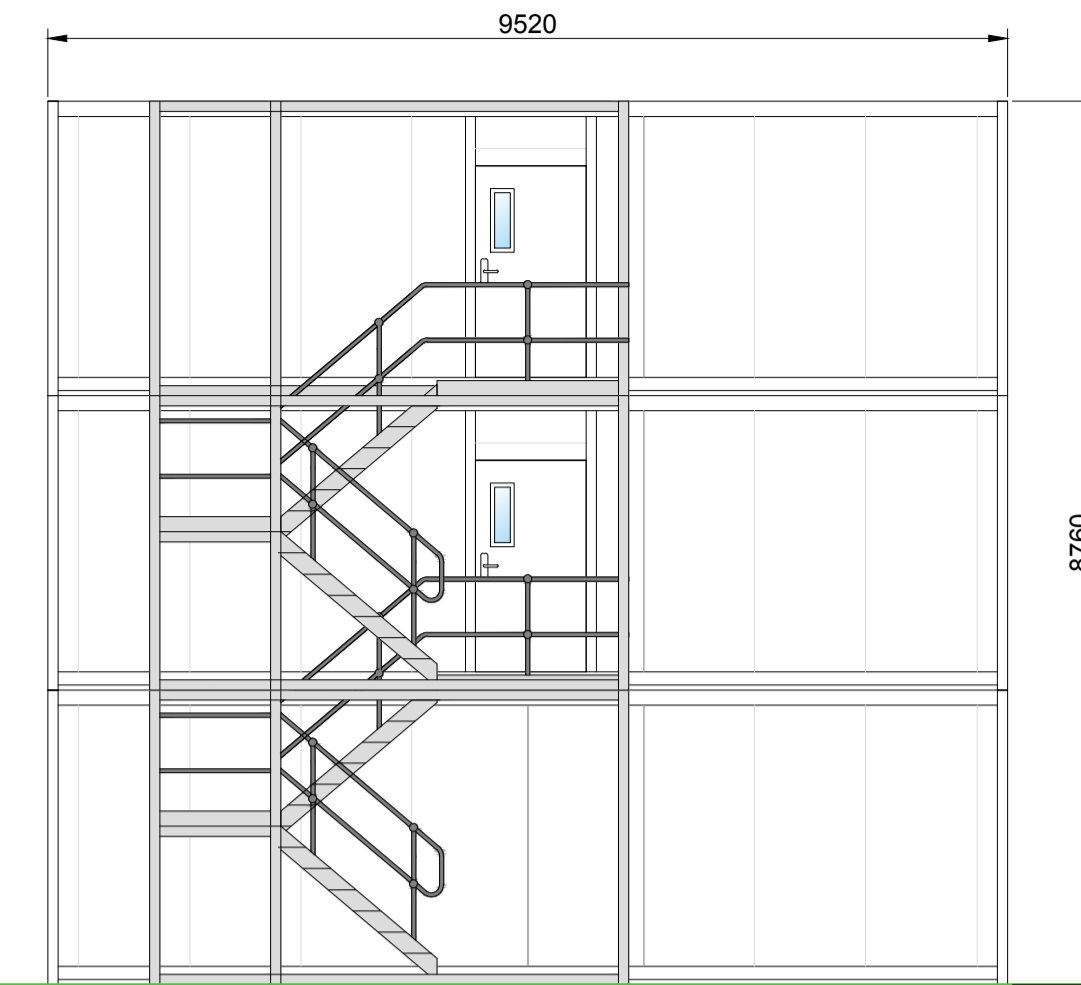
WEST ELEVATION
