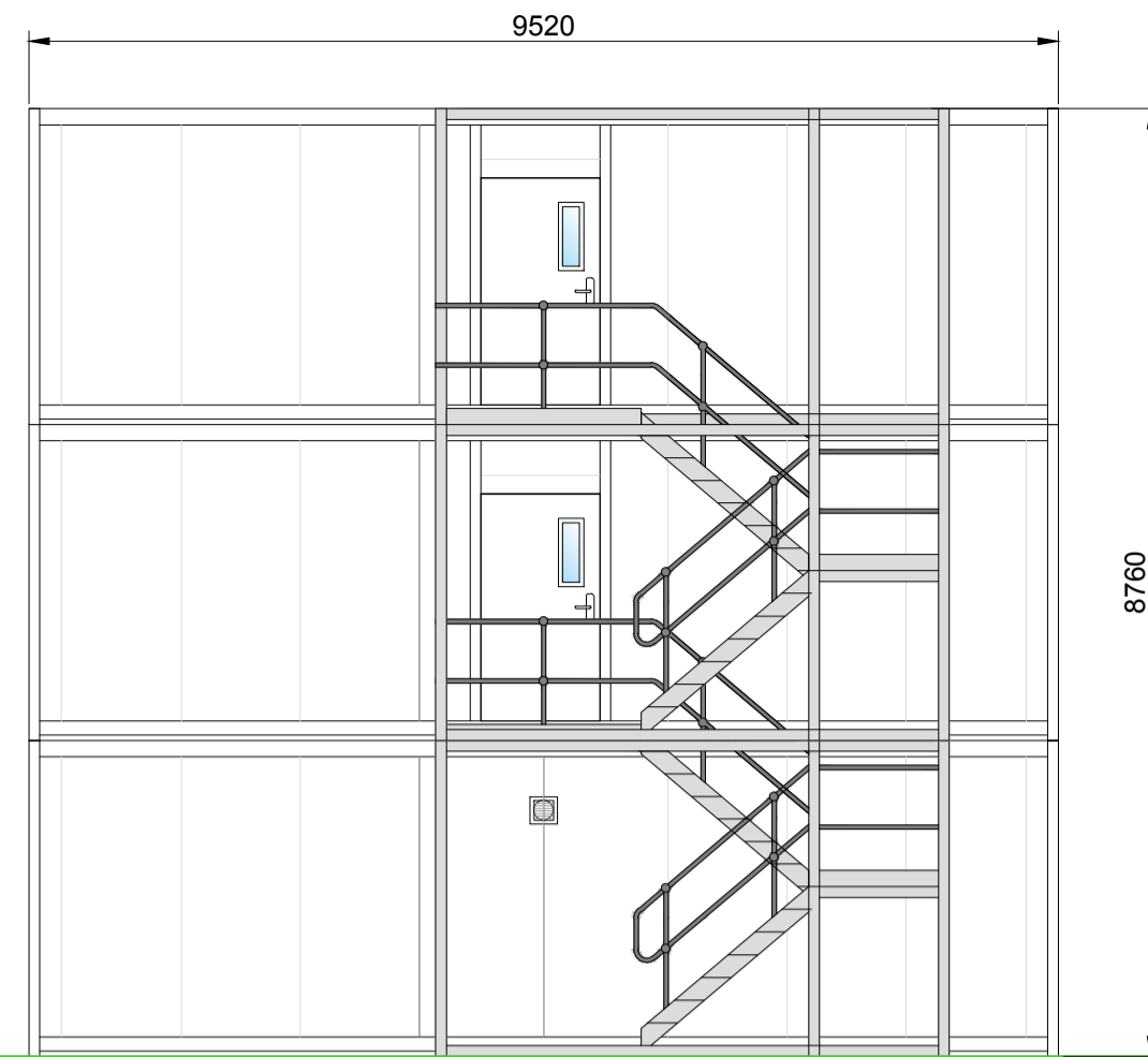
EAST ELEVATION
