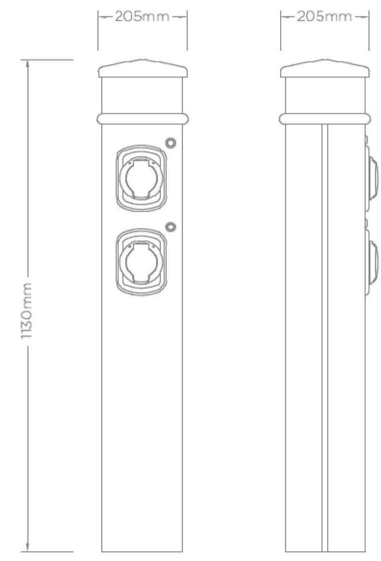
Car Charging Point to be Rolecserv BASICCHARGE:EV pedestal charging point. Refer to specification sheet for details.
