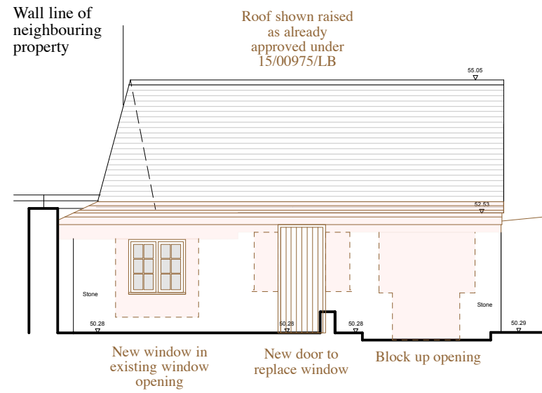
Elevation AA
