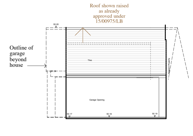
Elevation CC
