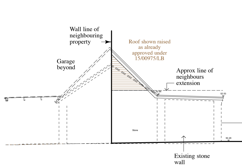
Elevation AA
