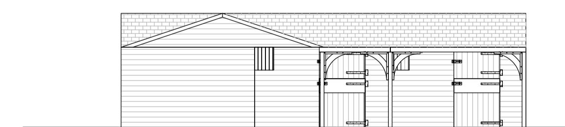
SOUTH ELEVATION 1:100
