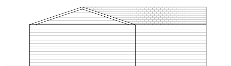
WEST ELEVATION 1:100
