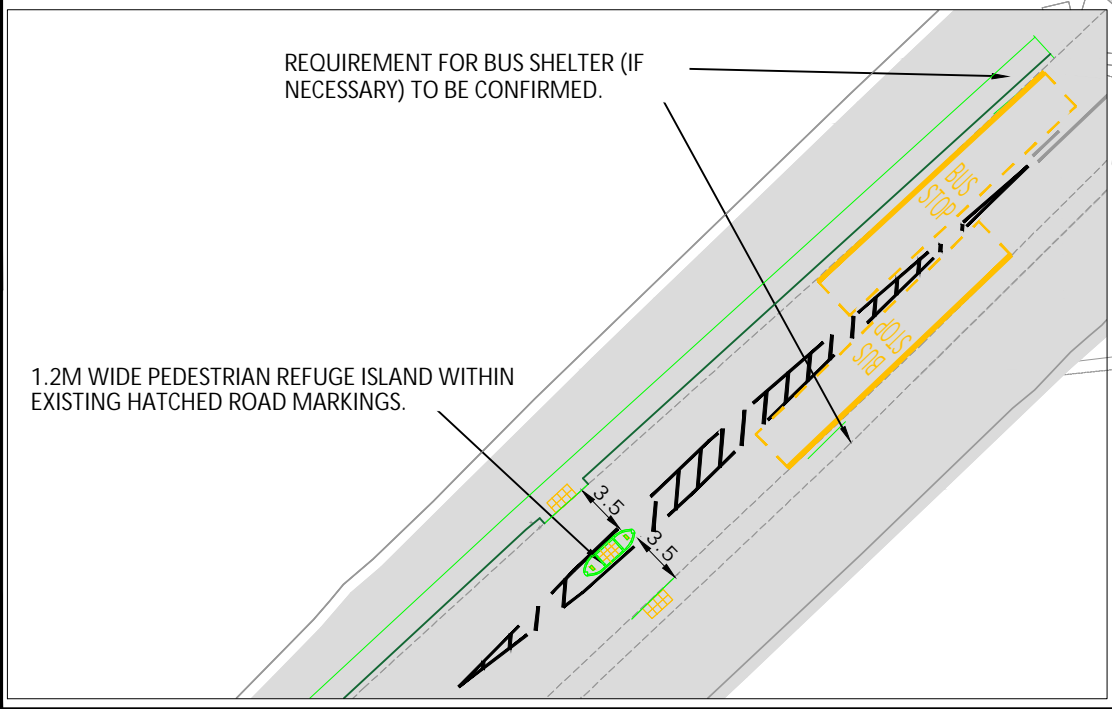
2M FOOTWAY/PED REFUGE WITH POTENTIAL BUS STOP LOCATIONS @ 1:500 SCALE
