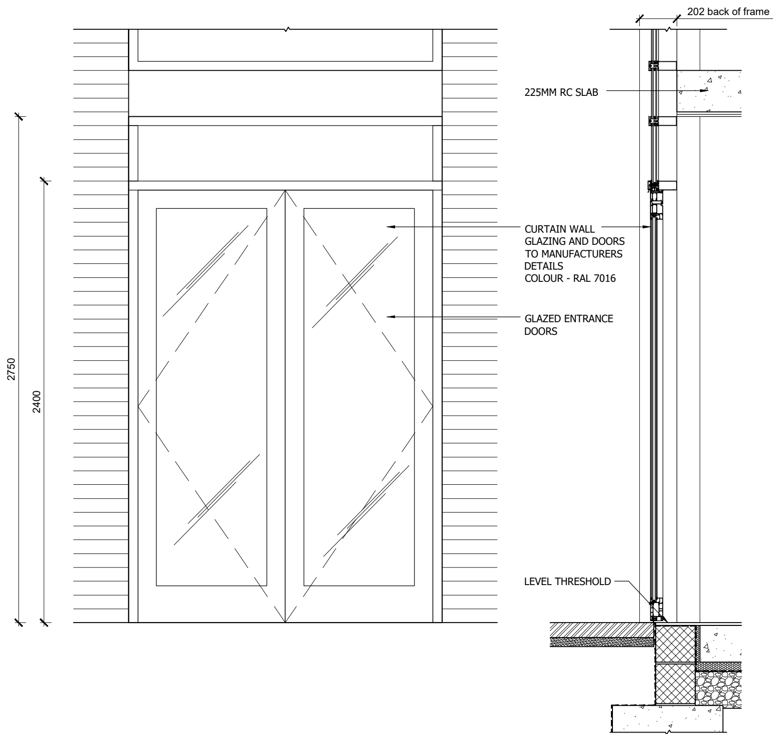
TYPICAL CURTAIN WALLING TO FLAT ENTRANCE LOBBIES
