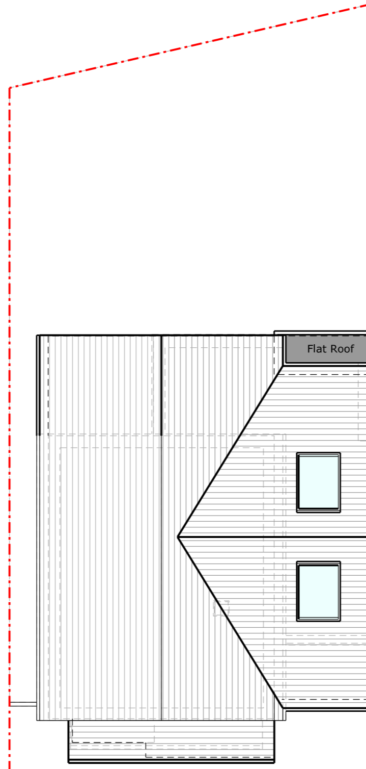
Roof Plan
