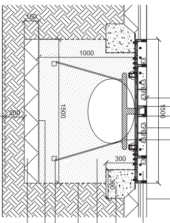
TP-H-A Tree pit detail: Primary Road - Castle tree grille (or similar approved)
