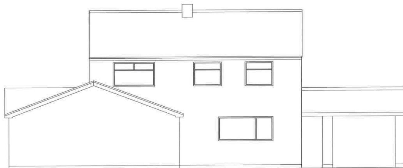
Ex. Rear Elevation
