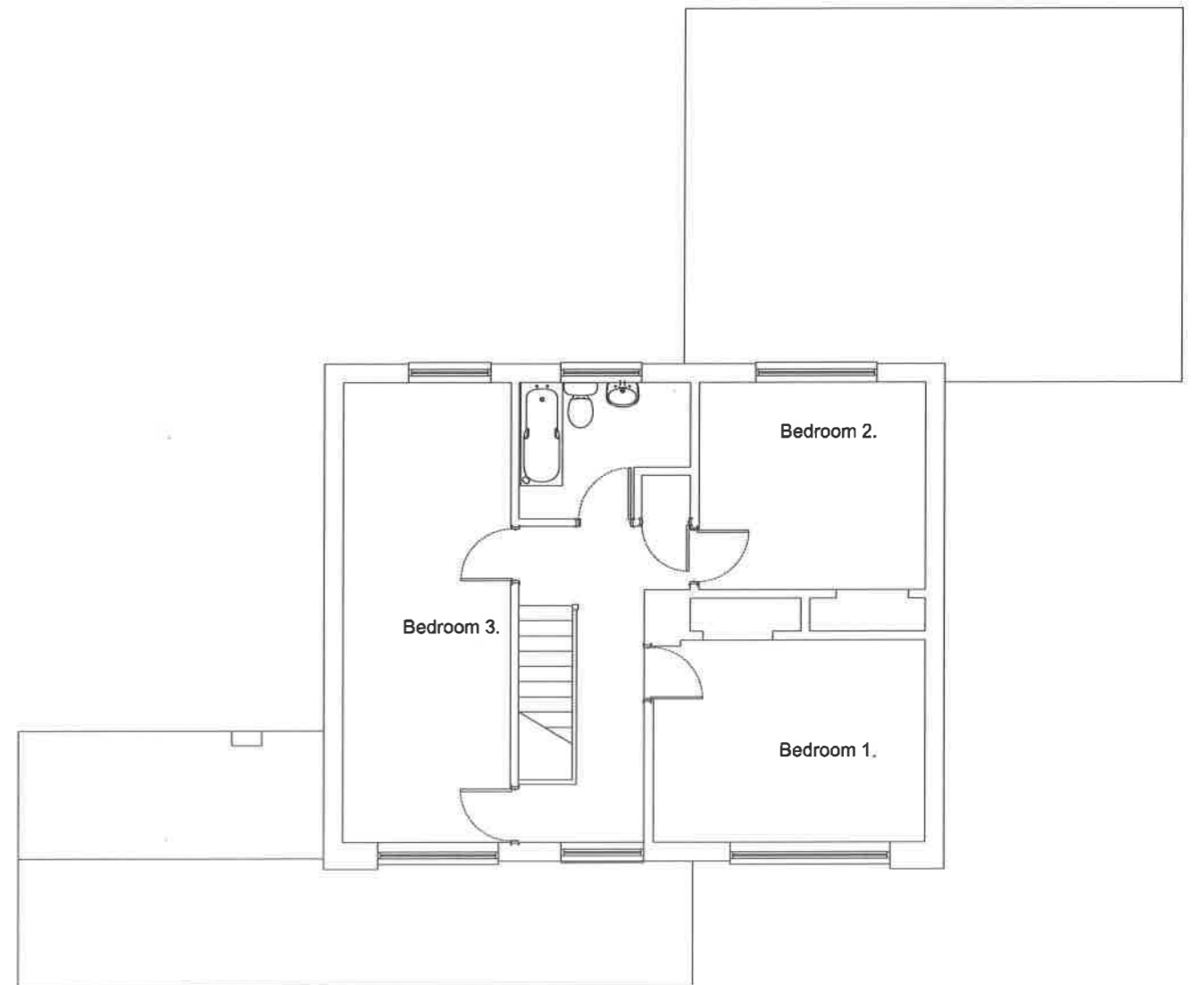
Existing 1st. Floor Plan
