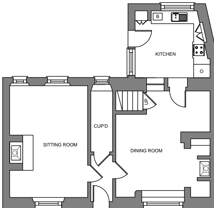
PREVIOUS GROUND FLOOR LAYOUT
