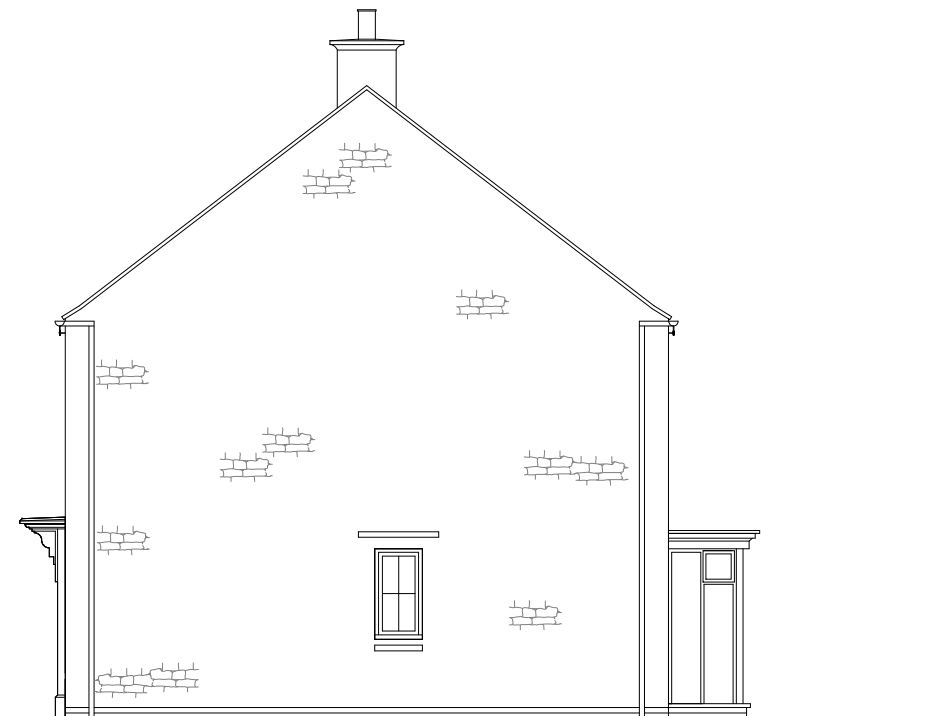
SIDE ELEVATION
