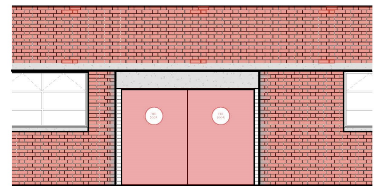
05 EXISTING ELEVATION 1:50
