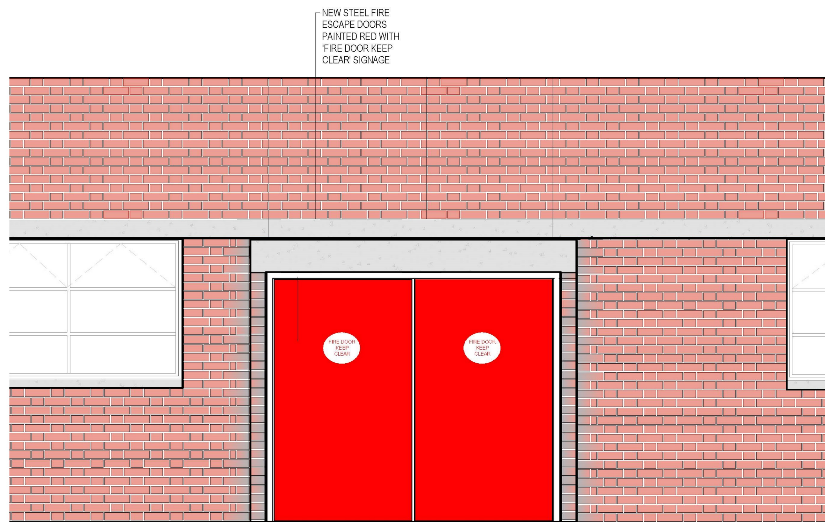
06 PROPOSED DOOR ELEVATION 1:20
