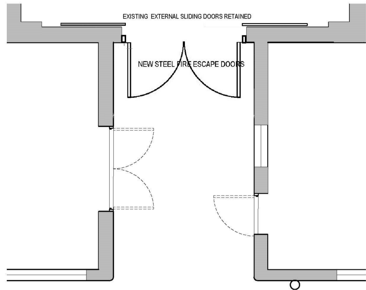
01 PROPOSED PLAN 1:50
