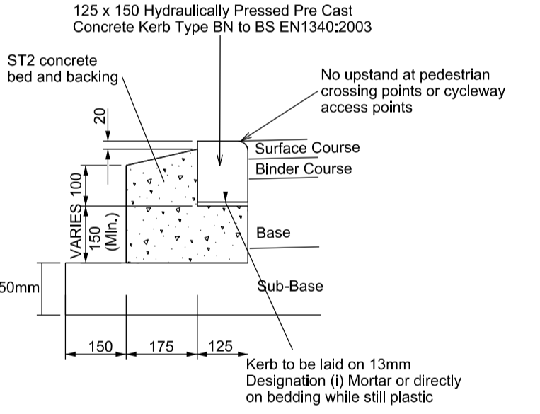
BULL- NOSED KERB (BN)
