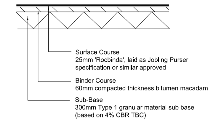
PRIVATE IMPERMEABLE DRIVE DETAIL
