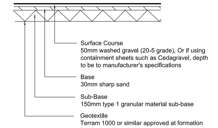
PRIVATE PERMEABLE DRIVE DETAIL
