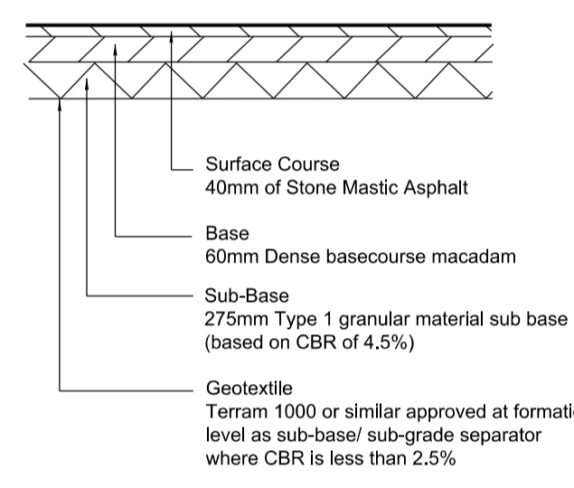
PRIVATE TARMAC DRIVE AND LIGHT DUTY ACCESS ROAD
