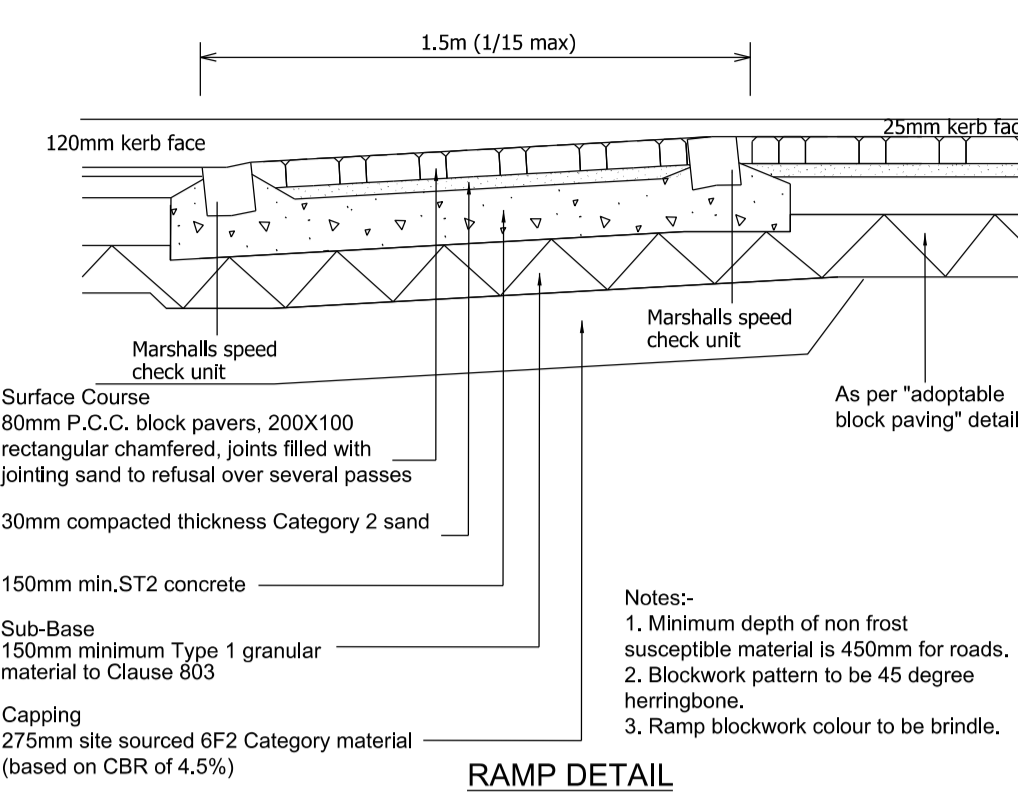
RAMP DETAIL
