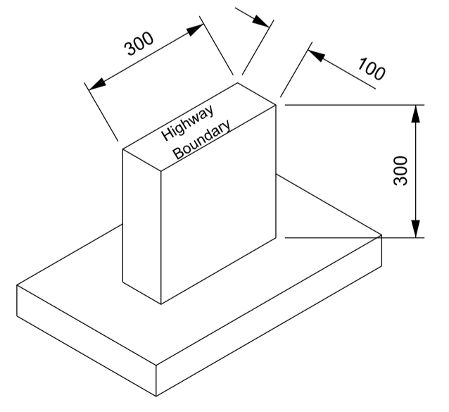
RC05 - HIGHWAY BOUNDARY MARKER DETAIL
