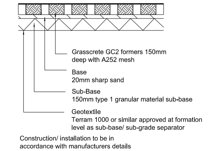
PRIVATE GRASSCRETE DETAIL
