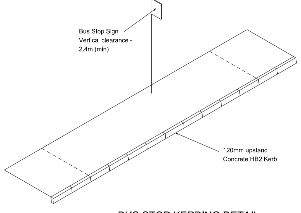
BUS STOP KERBING DETAIL
