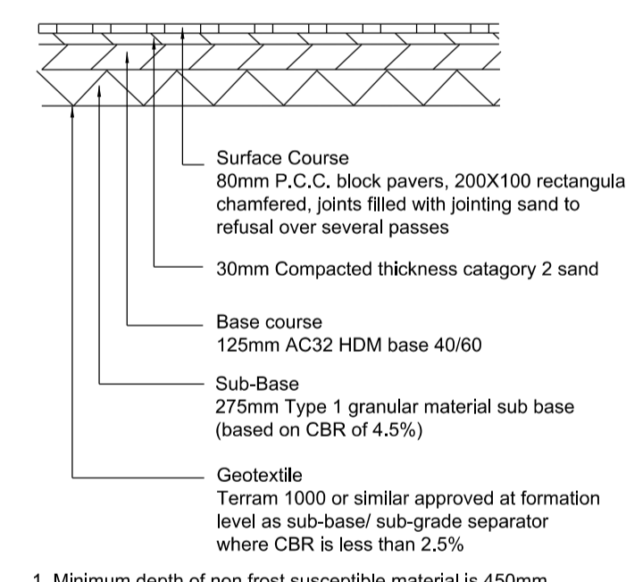
ADOPTABLE BLOCK PAVING/ PRIVATE BLOCK PAVING ACCESS
