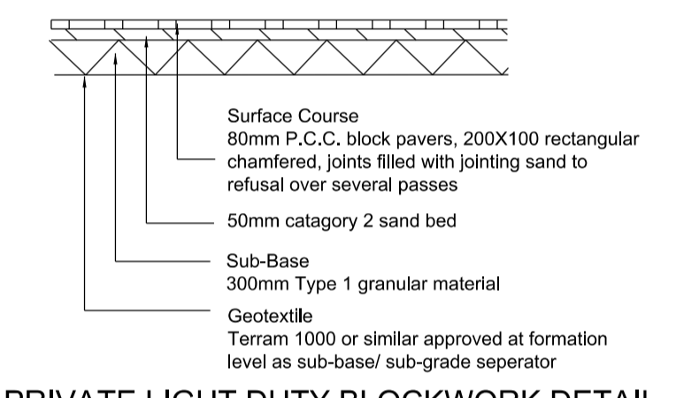
PRIVATE LIGHT DUTY BLOCKWORK DETAIL
