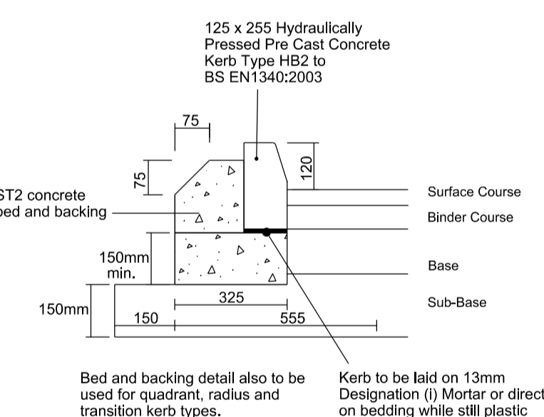
HALF BATTERED KERB (HB2)
