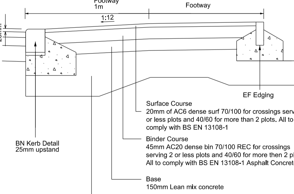
VEHICULAR CROSSING DETAIL
