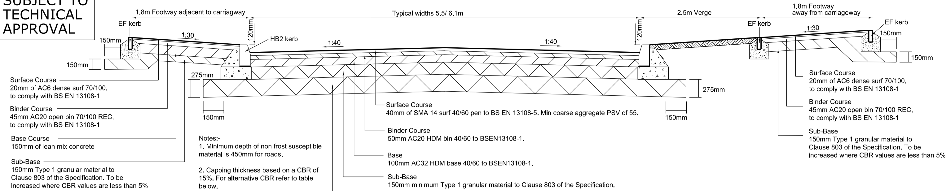
BLACKTOP CONSTRUCTION DETAIL
