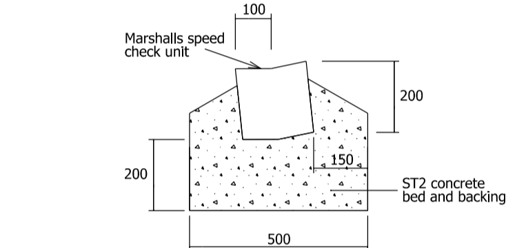
MARSHALLS SPEED CHECK UNIT (Or similar approved)
