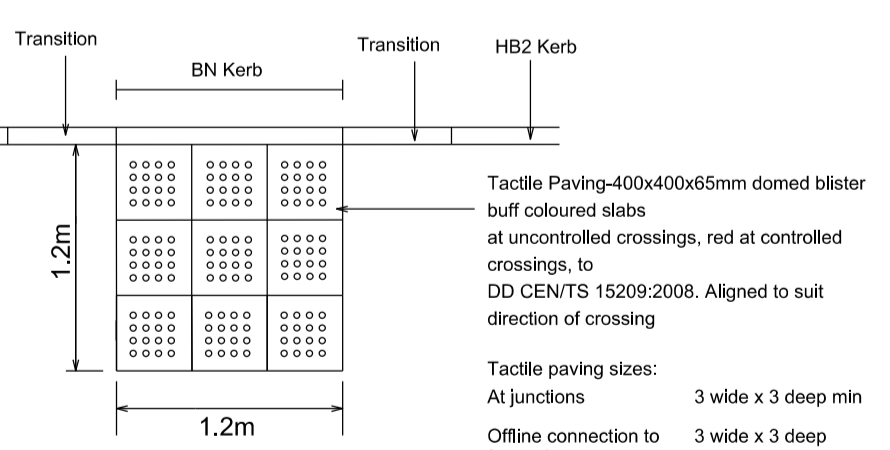
TACTILE CROSSING DETAIL
