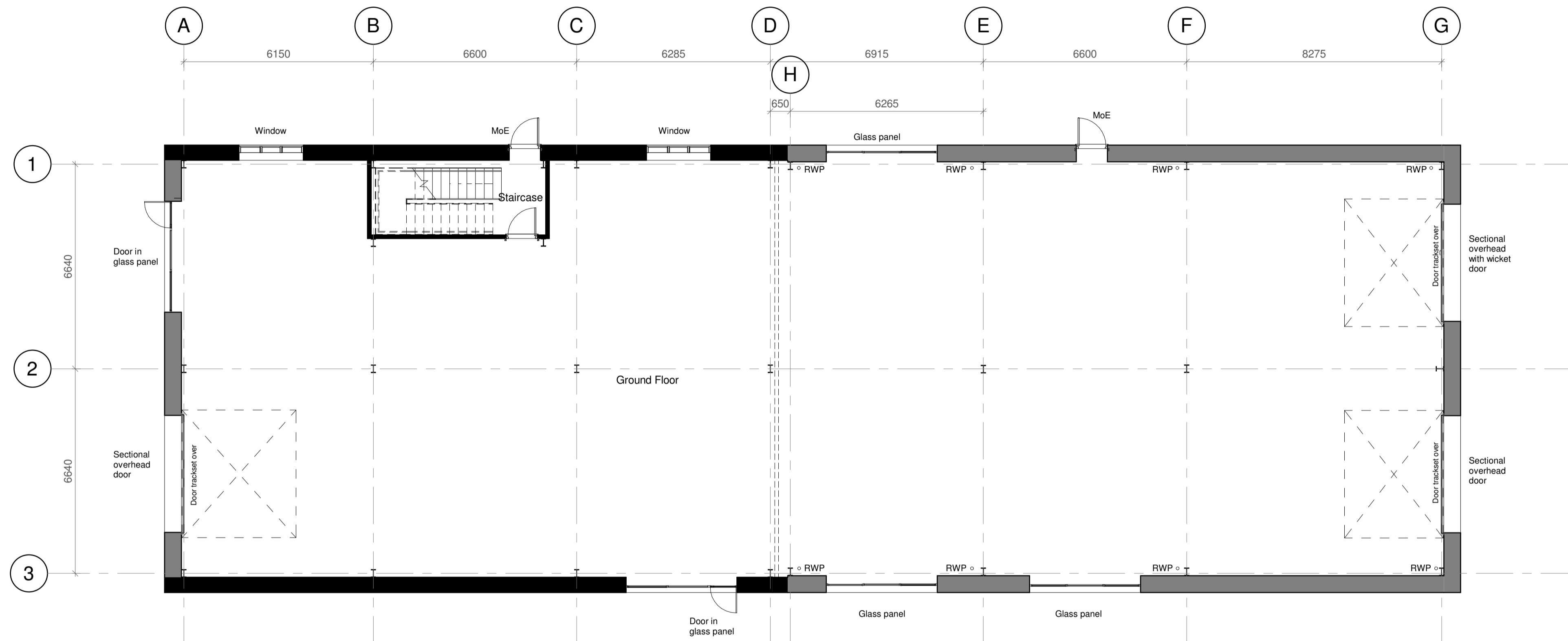
Ground Floor Plan 1 : 100
