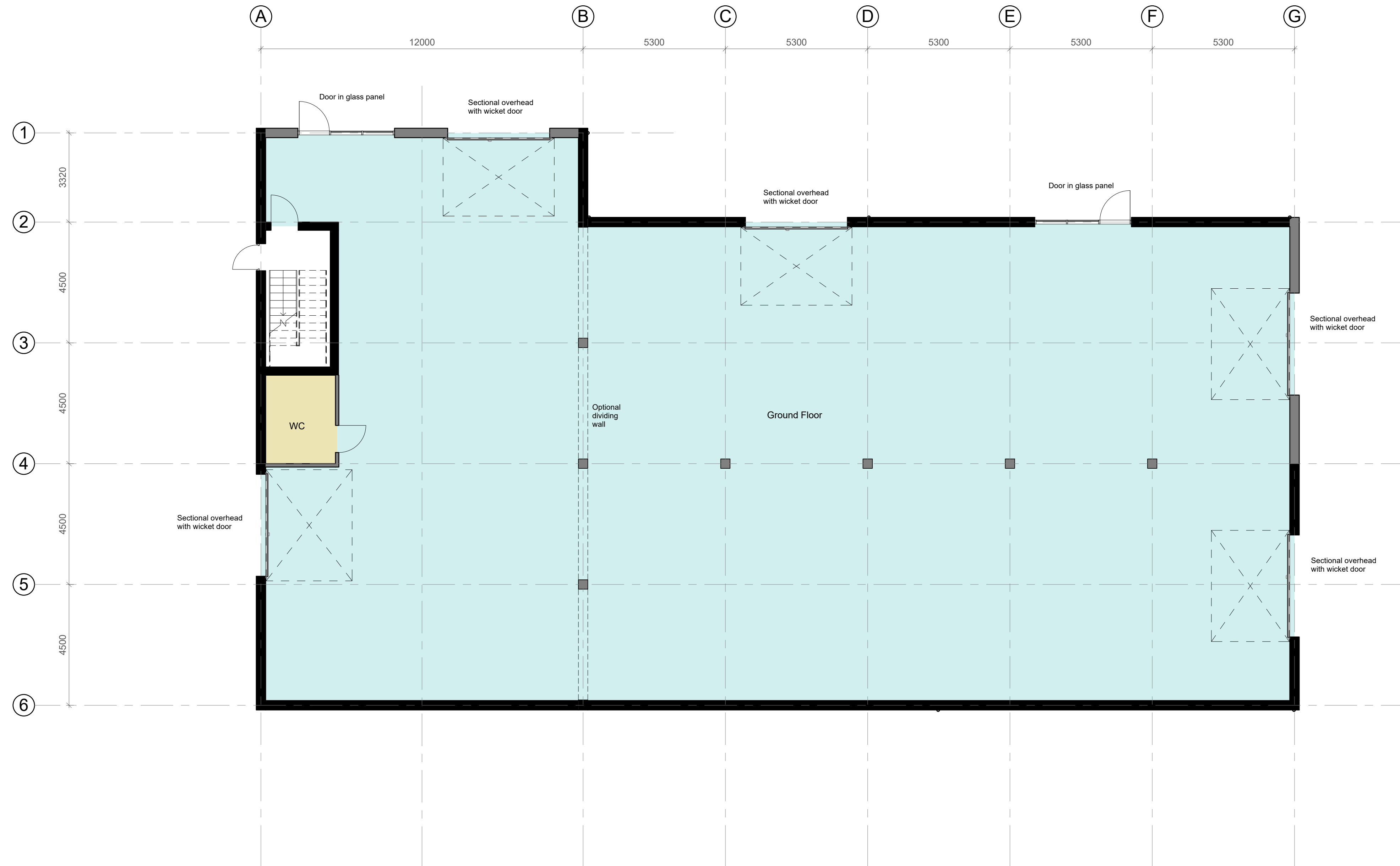
Ground Floor Plan 1 : 100
