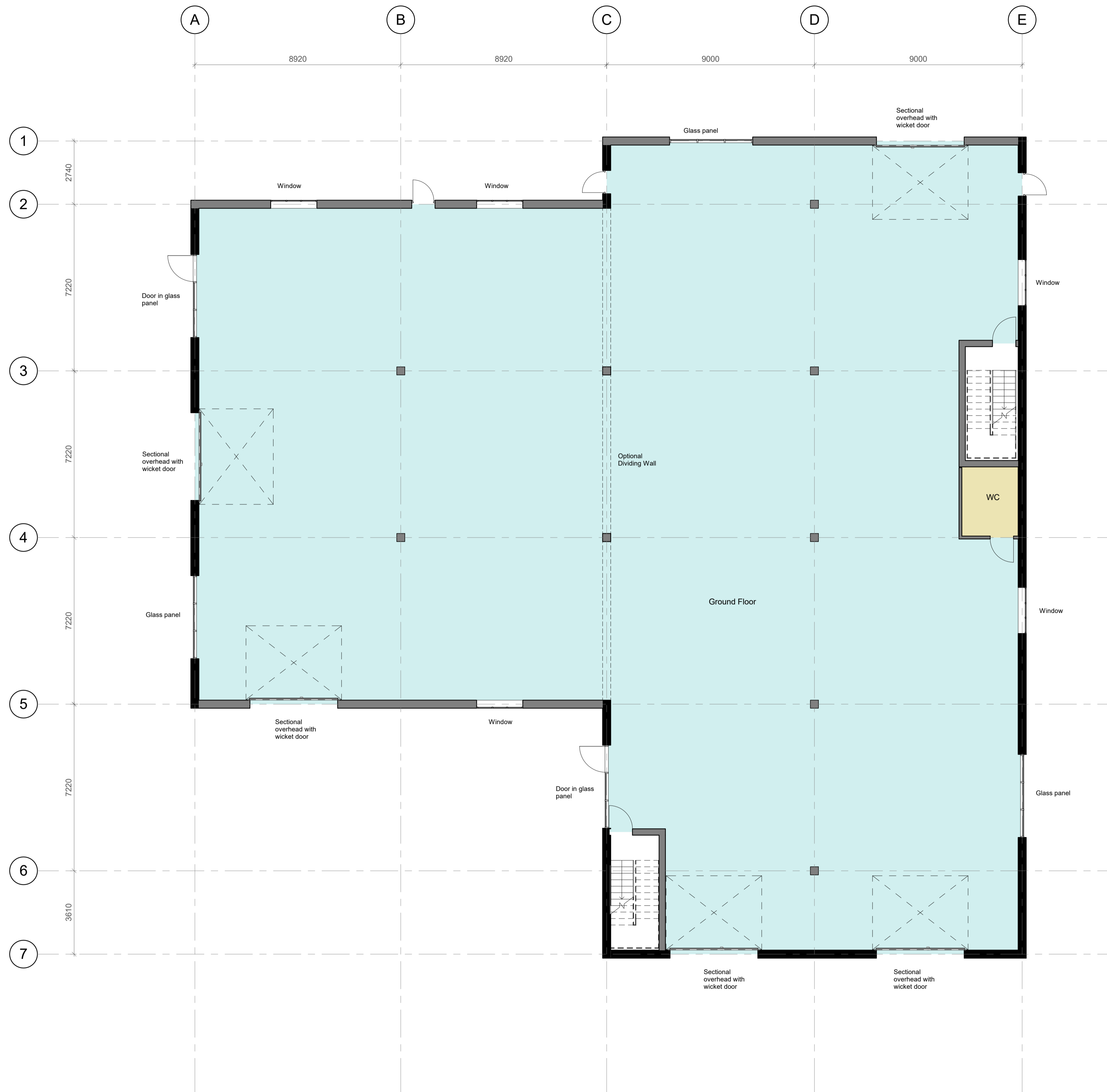
Ground Floor Plan 1 : 100
