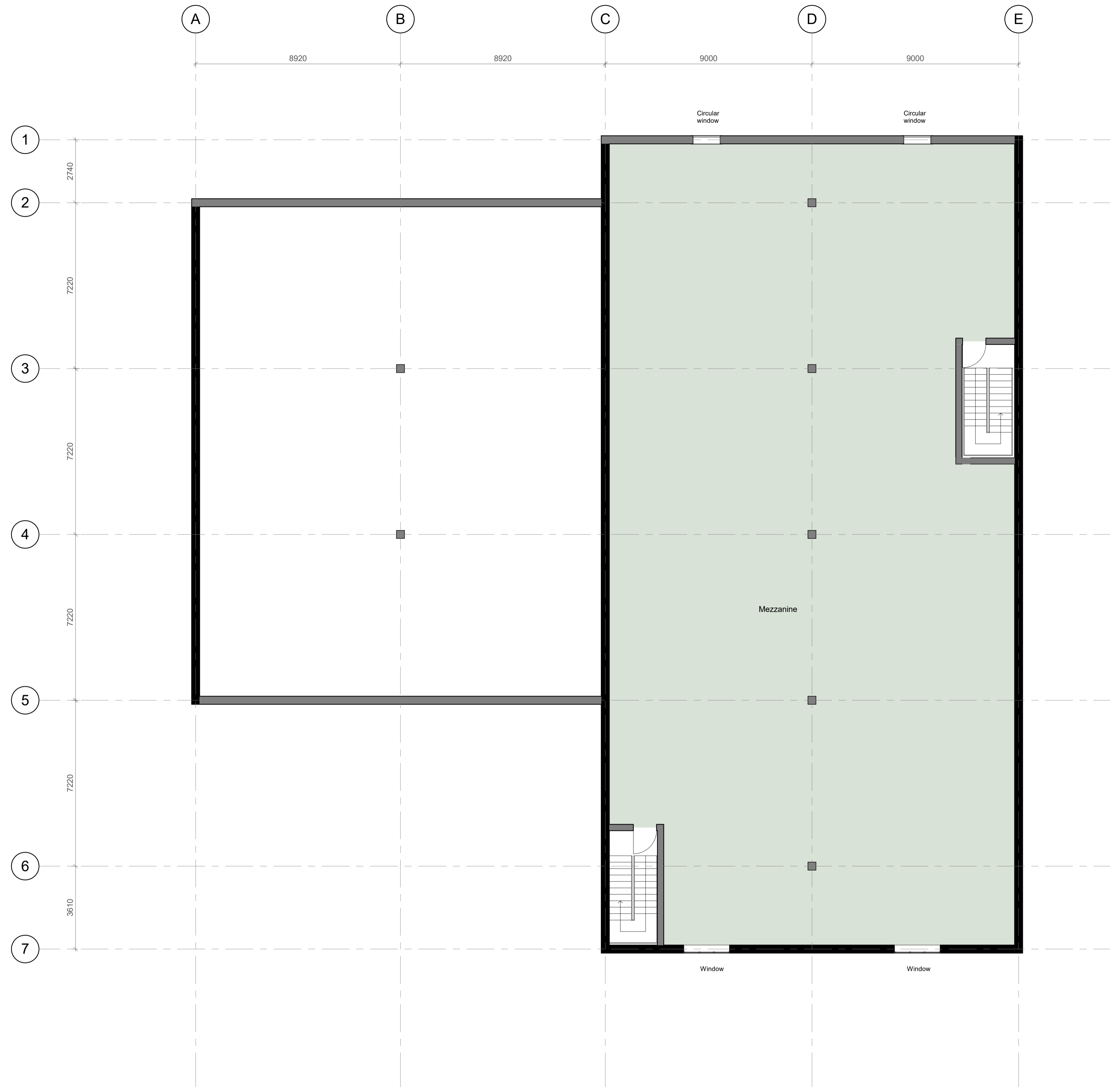
Mezzanine Floor Plan 1 : 100
