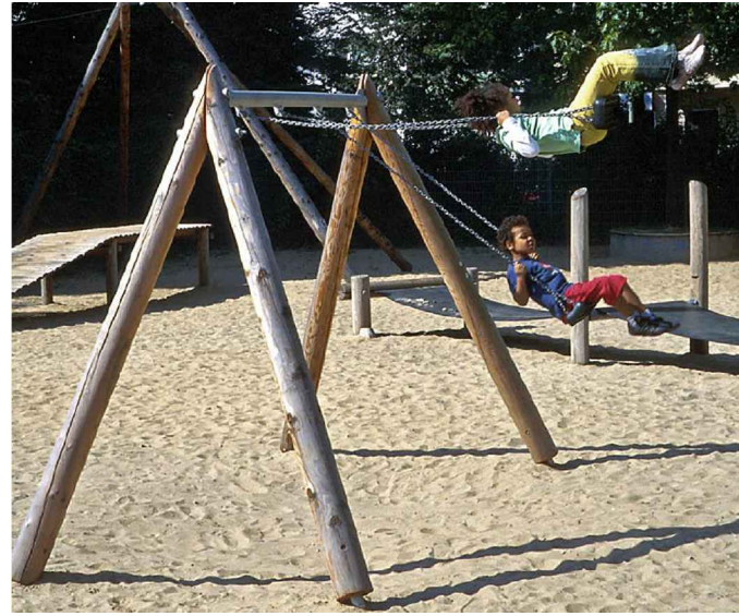
DOUBLE SWING Richter-Spielgeraete, Item 61280 with metal feet.
