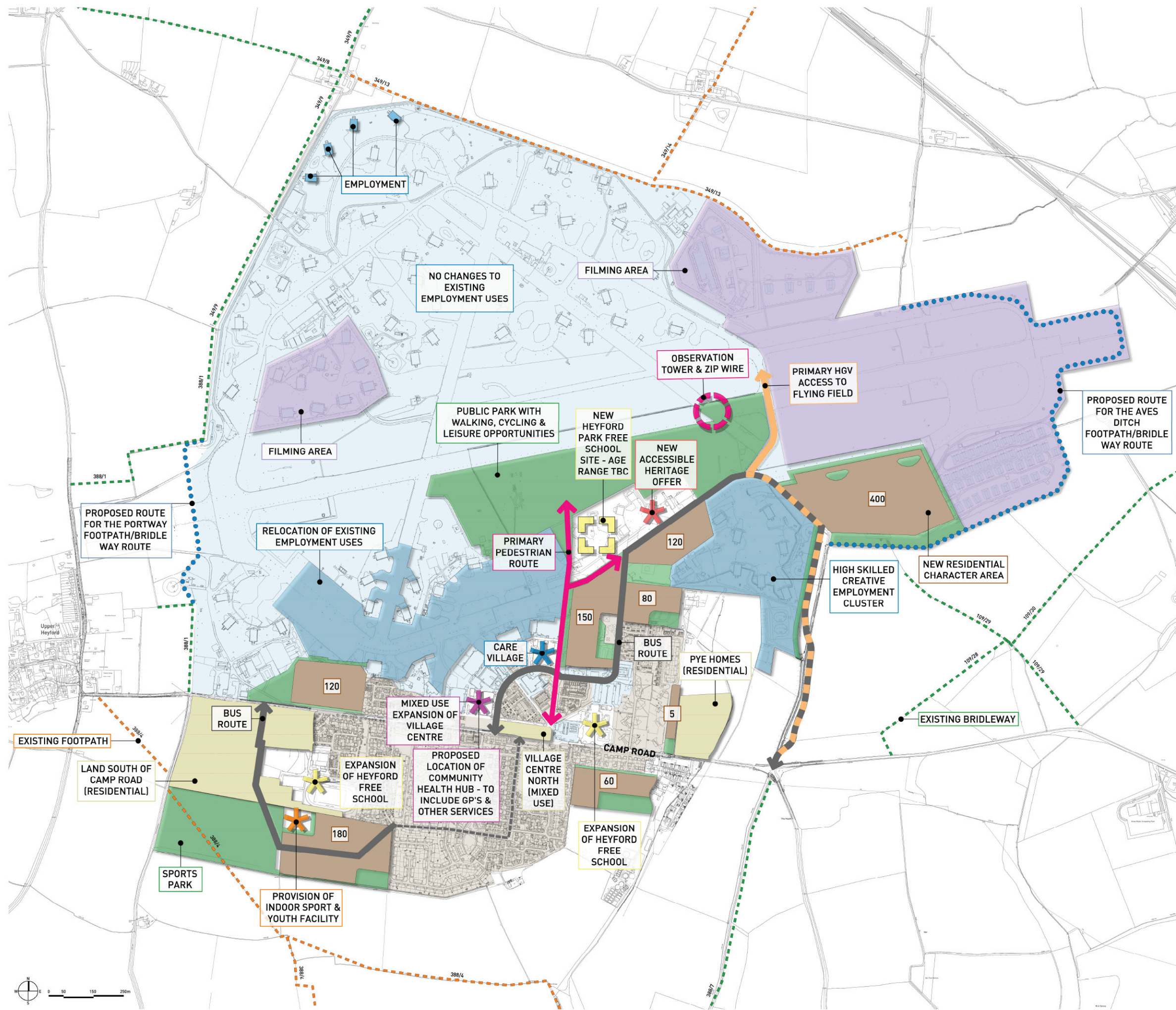
FIGURE 4.9 Heyford Concept Masterplan DRWG No: P16-0631_87 REV: _ Date: 23/03/2018 Sheet: 3/3 Scale: 1:12,500 @ A3
