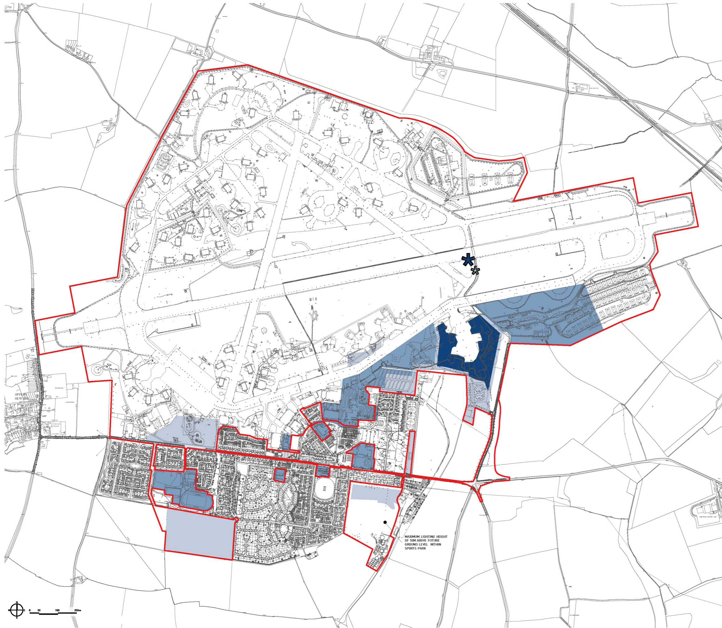
FIGURE 4.3a Building Height Parameters Plan
