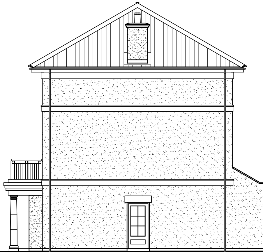
SIDE ELEVATION
