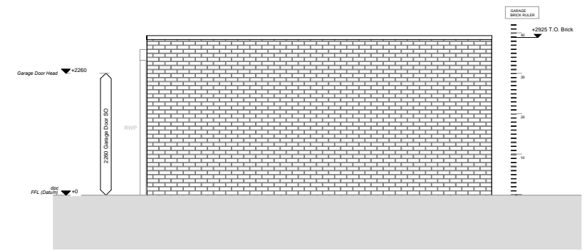
Side Elevation 2
