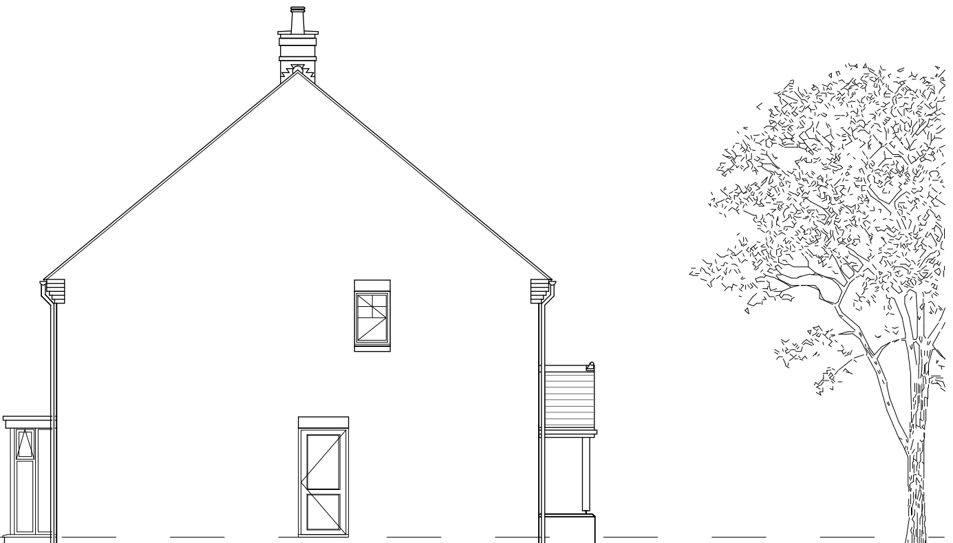
SIDE ELEVATION
