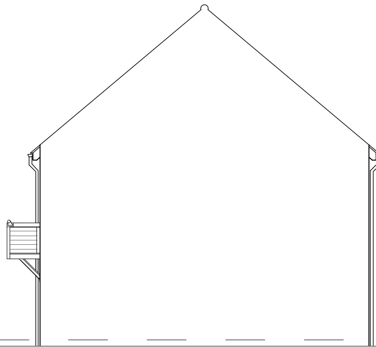
SIDE ELEVATION
