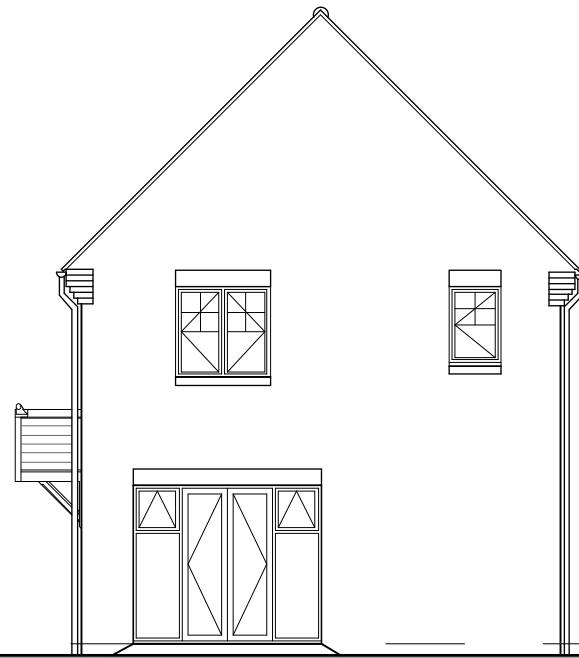
SIDE ELEVATION
