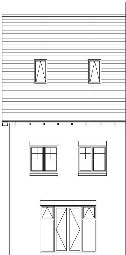
REAR ELEVATION
