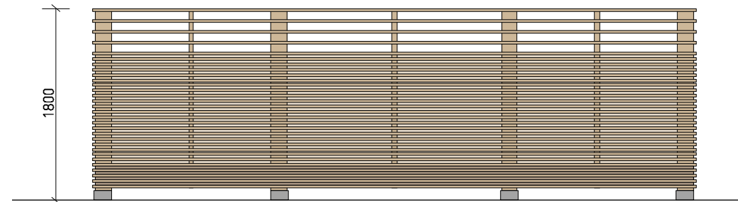
FRONT ELEVATION
