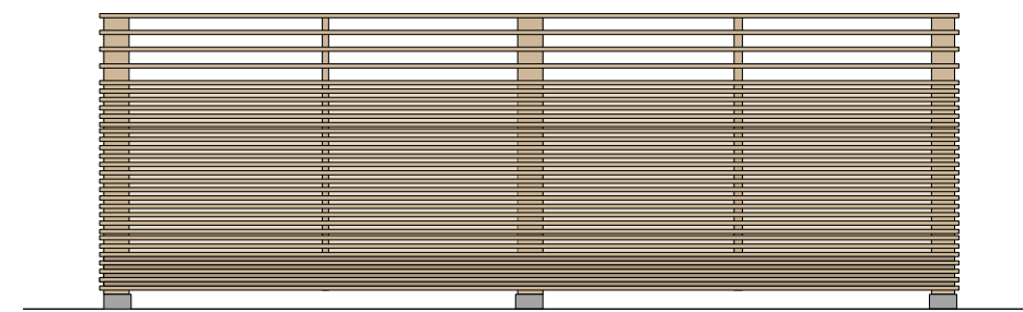
SIDE ELEVATION
