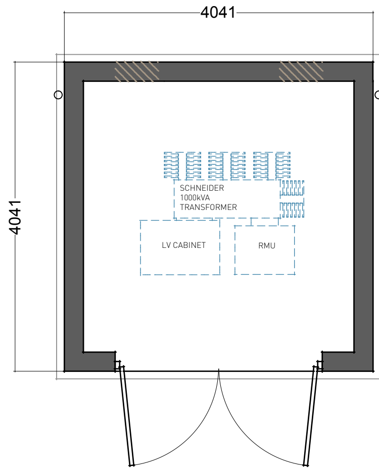
FLOOR PLAN
