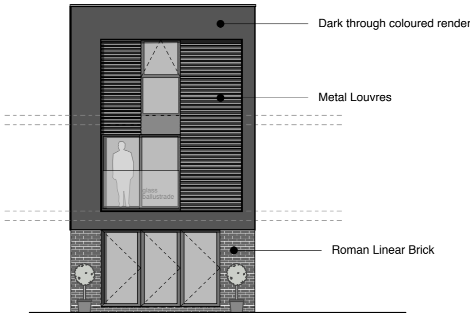
Rear Elevation (NORTH)
