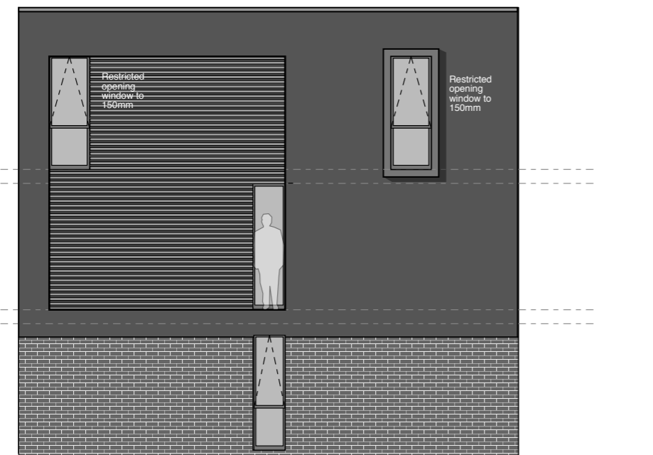
West Elevation
