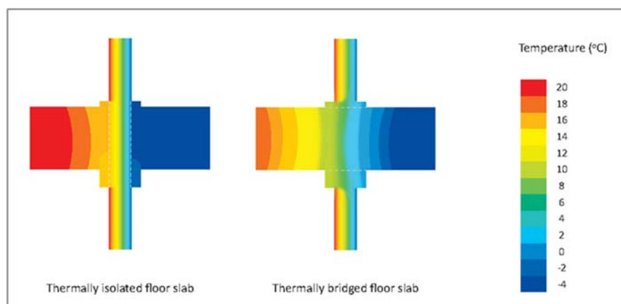
Figure 3: Thermal Bridging (SCI P380 2012)
