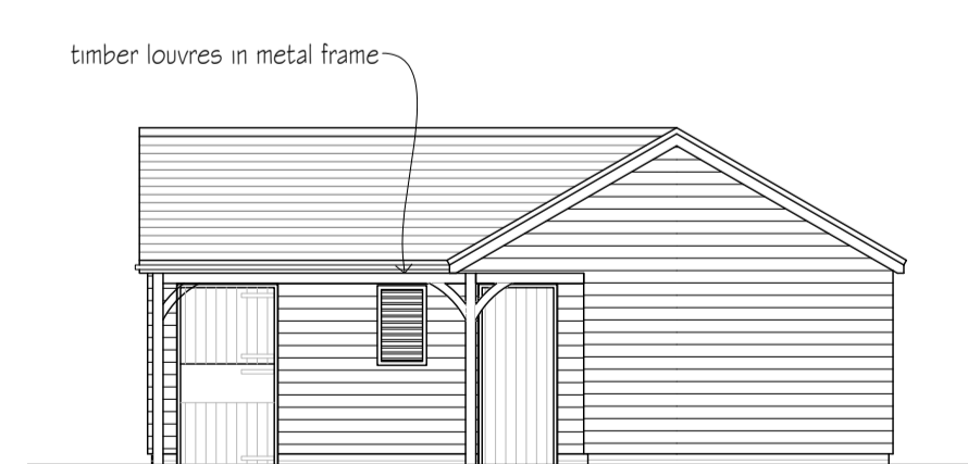
NORTH-WEST ELEVATION 1:100
