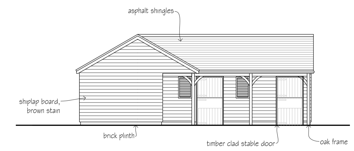
NORTH-EAST ELEVATION 1:100
