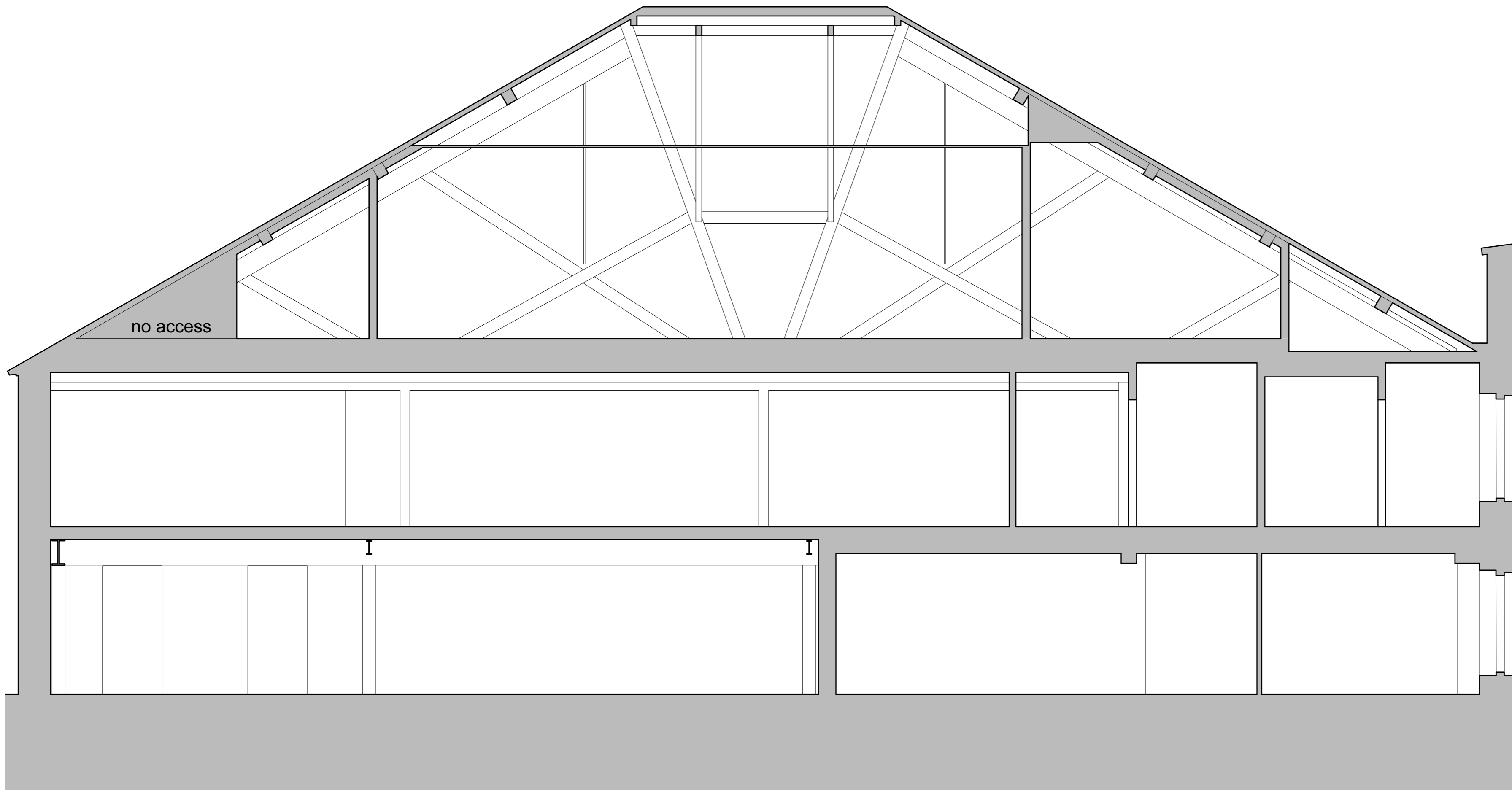
SECTION B-B AS EXISTING
