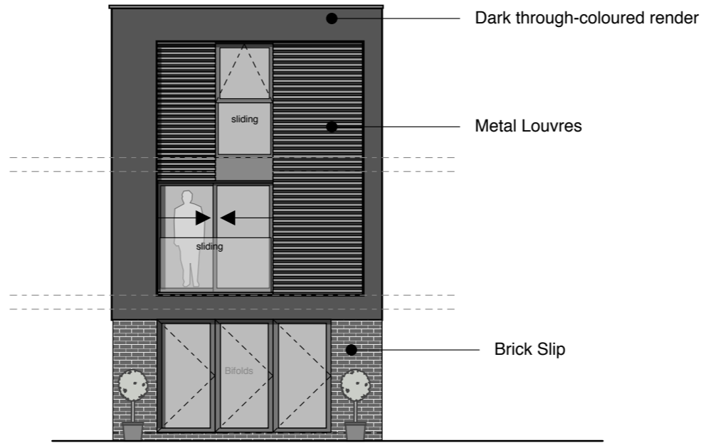
Rear Elevation (NORTH)
