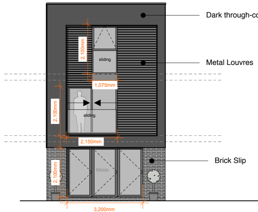
Rear Elevation (NORTH)
