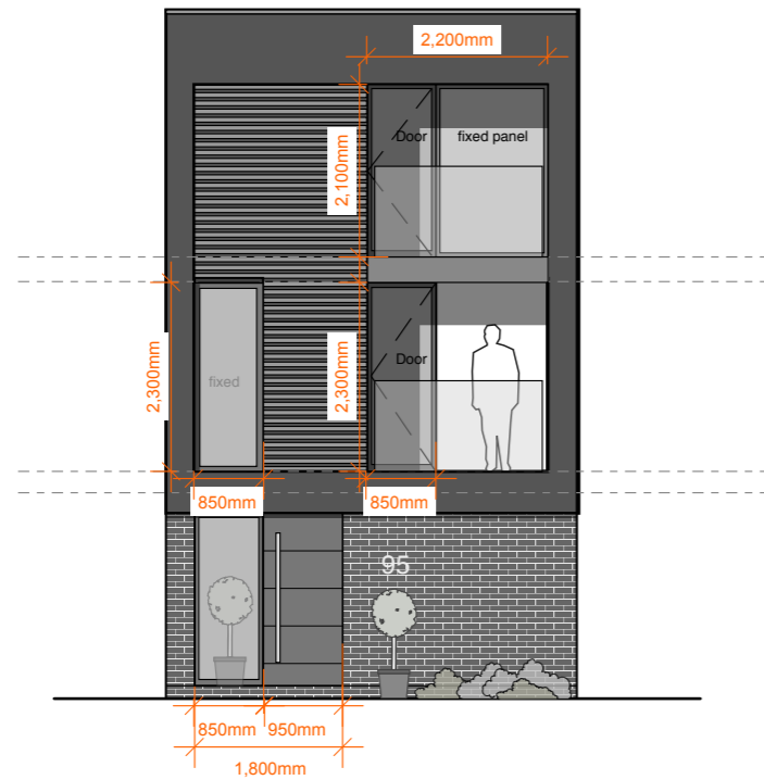
Street Elevation (SOUTH)
