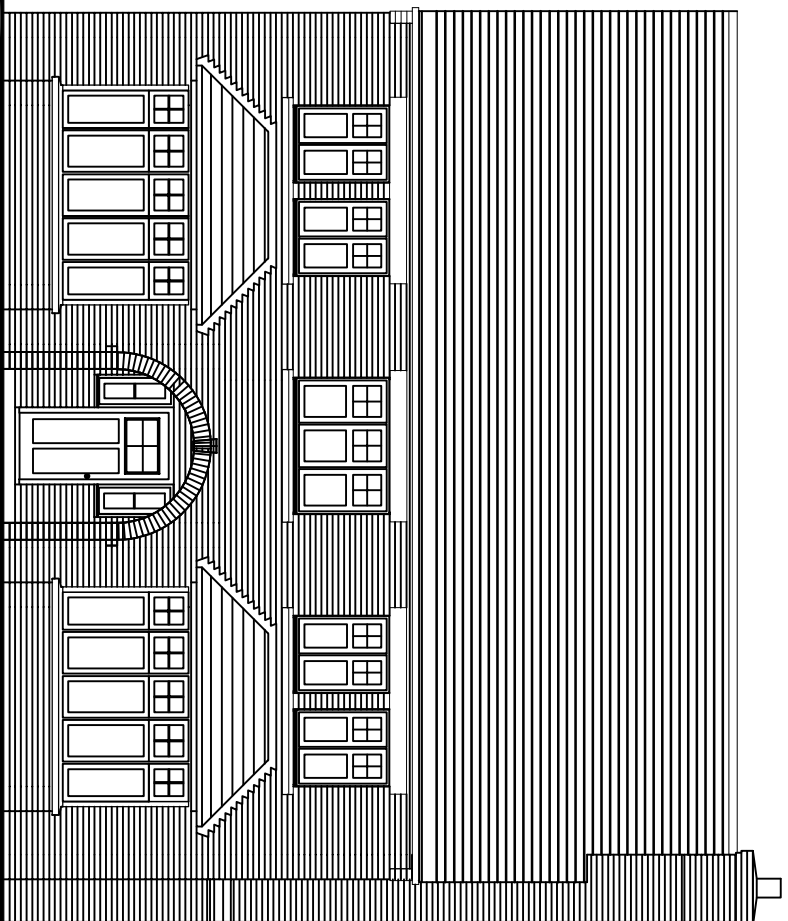
FRONT ELEVATION
