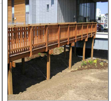
PROPOSED TIMBER BRIDGE. To be FSC hardwood, 'Woodscape Hardwood Timber Vertical Infill Bridge' or equal approved.
