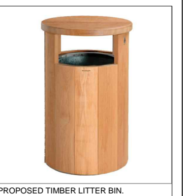
PROPOSED TIMBER LITTER BIN. To be FSC hardwood, 'Woodscape LBR 90' or equal approved.
