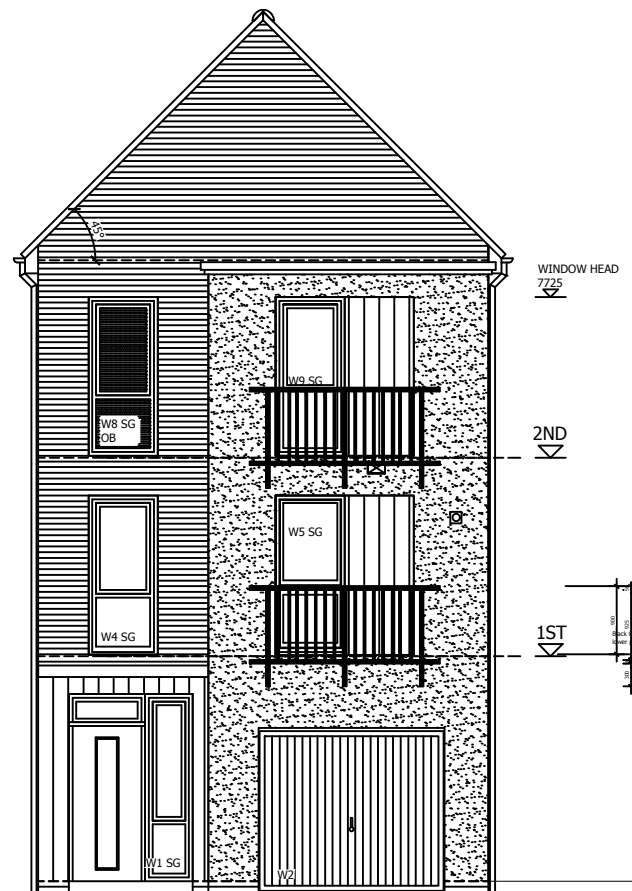
FRONT ELEVATION PLOTS 365 & 369
