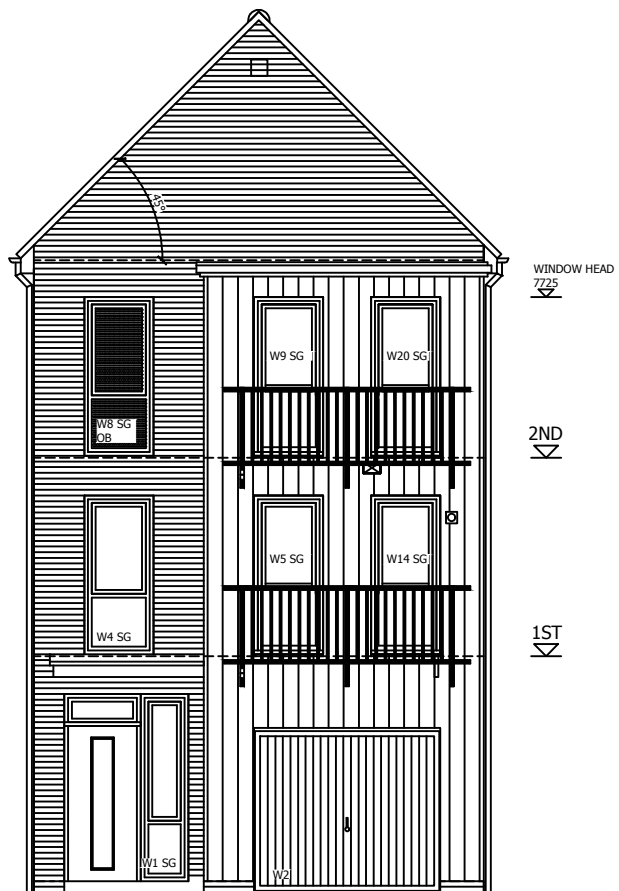
FRONT ELEVATION PLOTS 405 & 408
