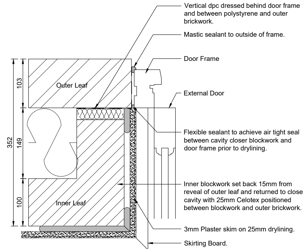
External door Jamb with returned blockwork Detail.
