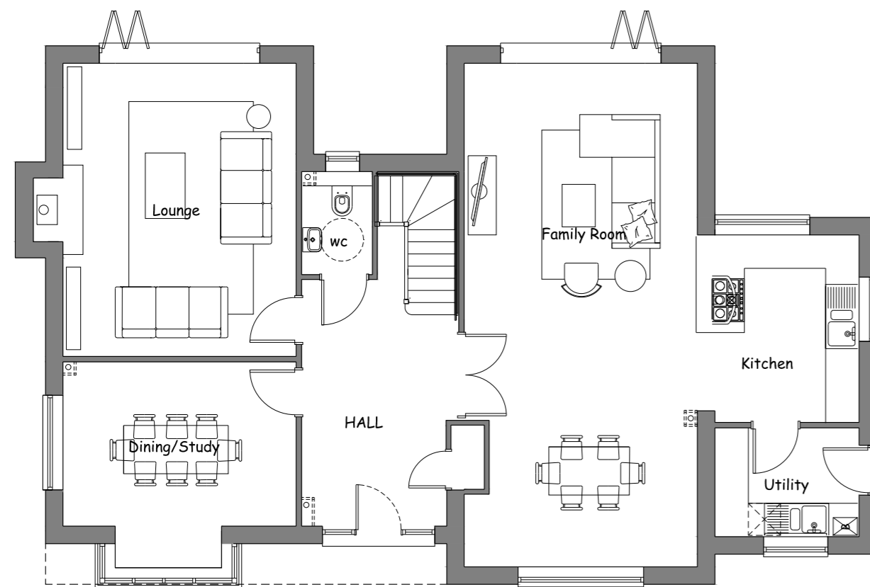
Ground Floor
