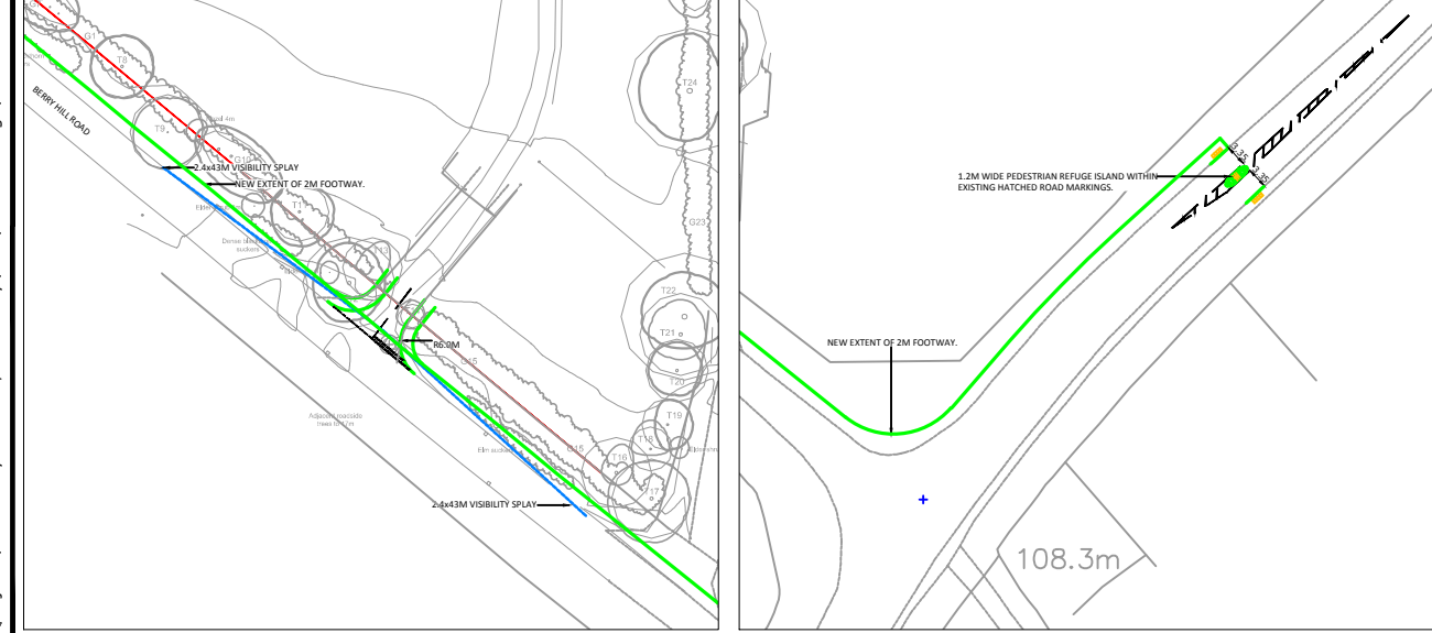
SITE ACCESS JUNCTION @ 1:1250 SCALE 2M FOOTWAY/PED REFUGE @ 1:1250 SCALE
