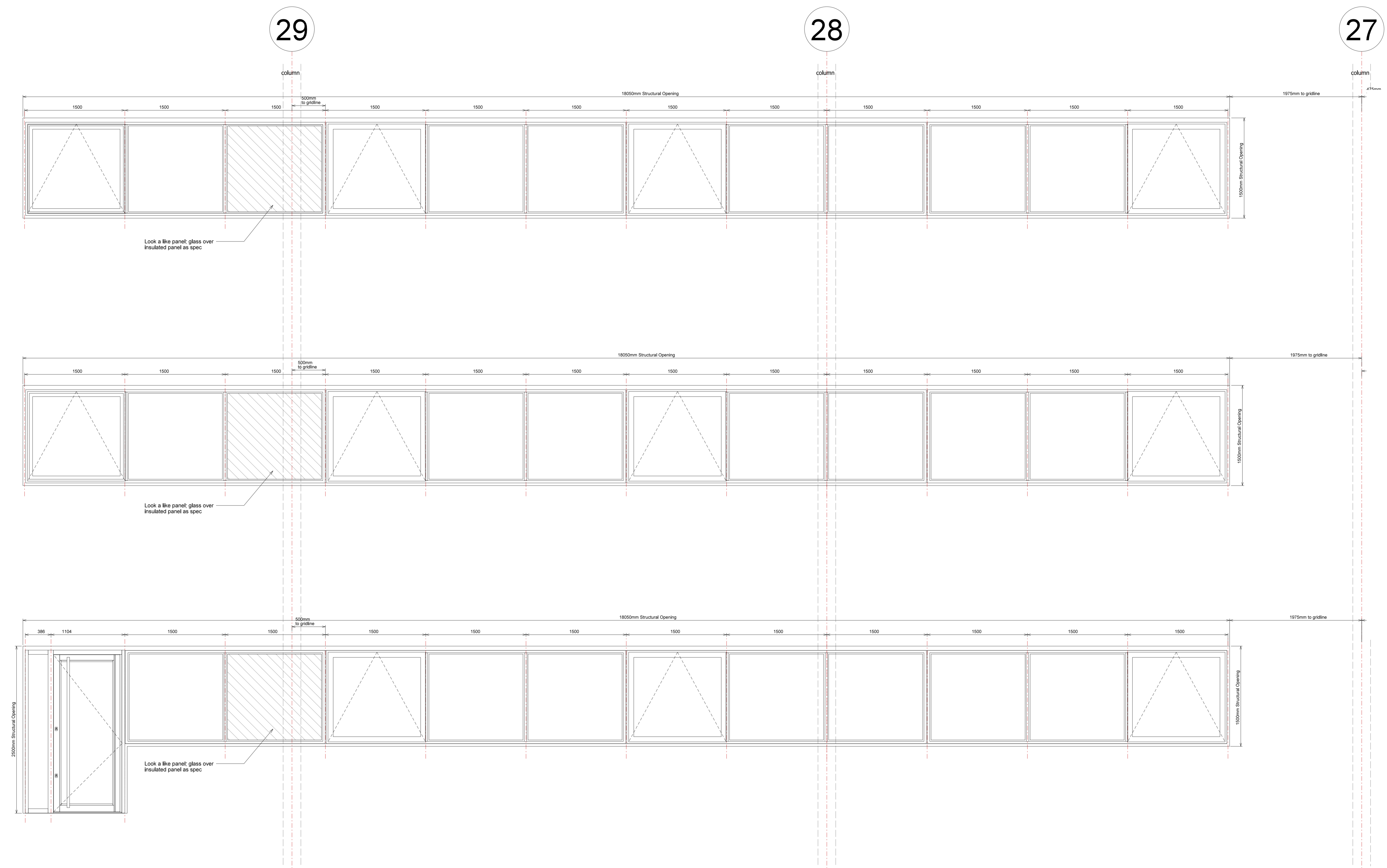
01 UNIT 1A WINDOWS 1503 Elevations
