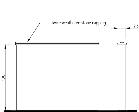
1800mm High Screen Wall
