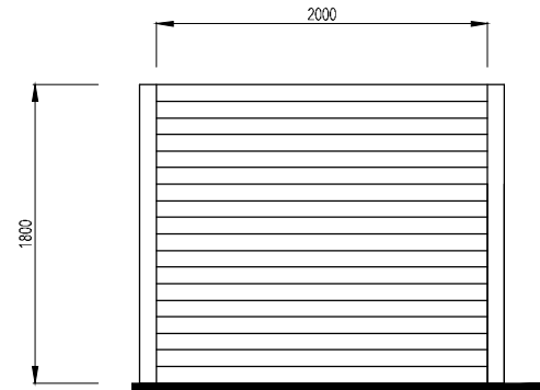
1800mm High Plot Division Panel Fence
