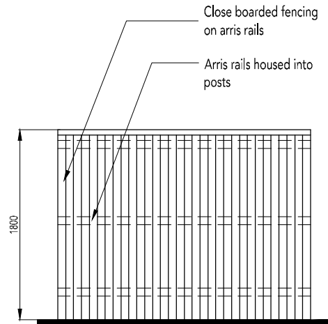
1800mm High Close Board Fence
