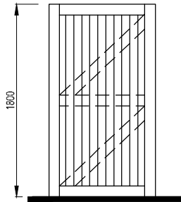
1800mm High Timber Matchboard Access Gate 1800mm
