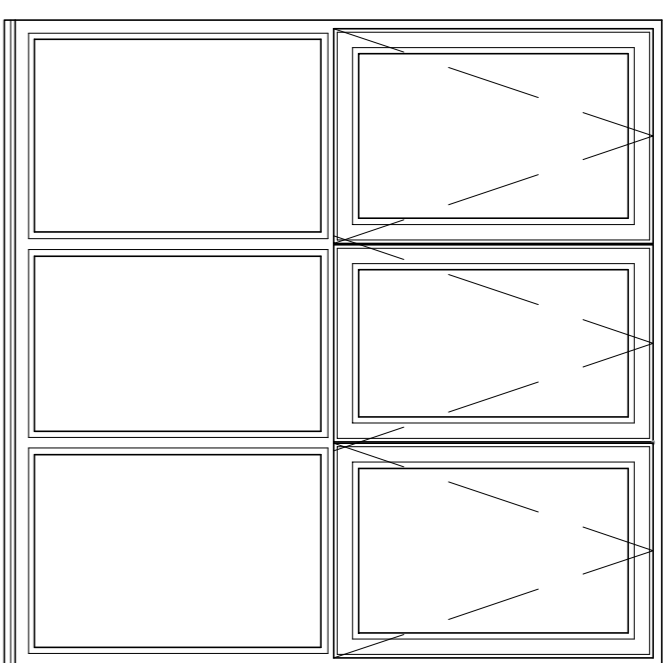
Window Style - Type 1 3 bay with 3 top openers
