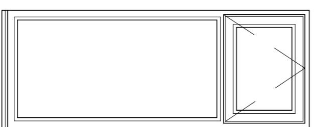
Window Style - Type 7 Single bay with top opener
