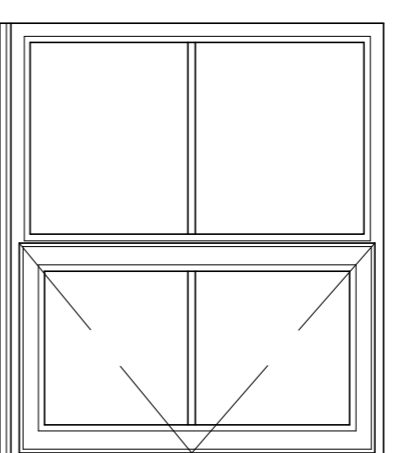
Window Style - Type 6 2 bay with horizontal bar and 1 full height side opener
