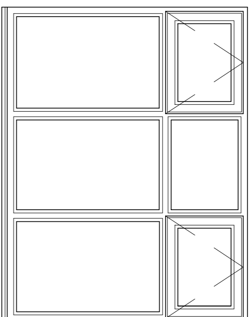
Window Style - Type 2 3 bay with 2 top openers
