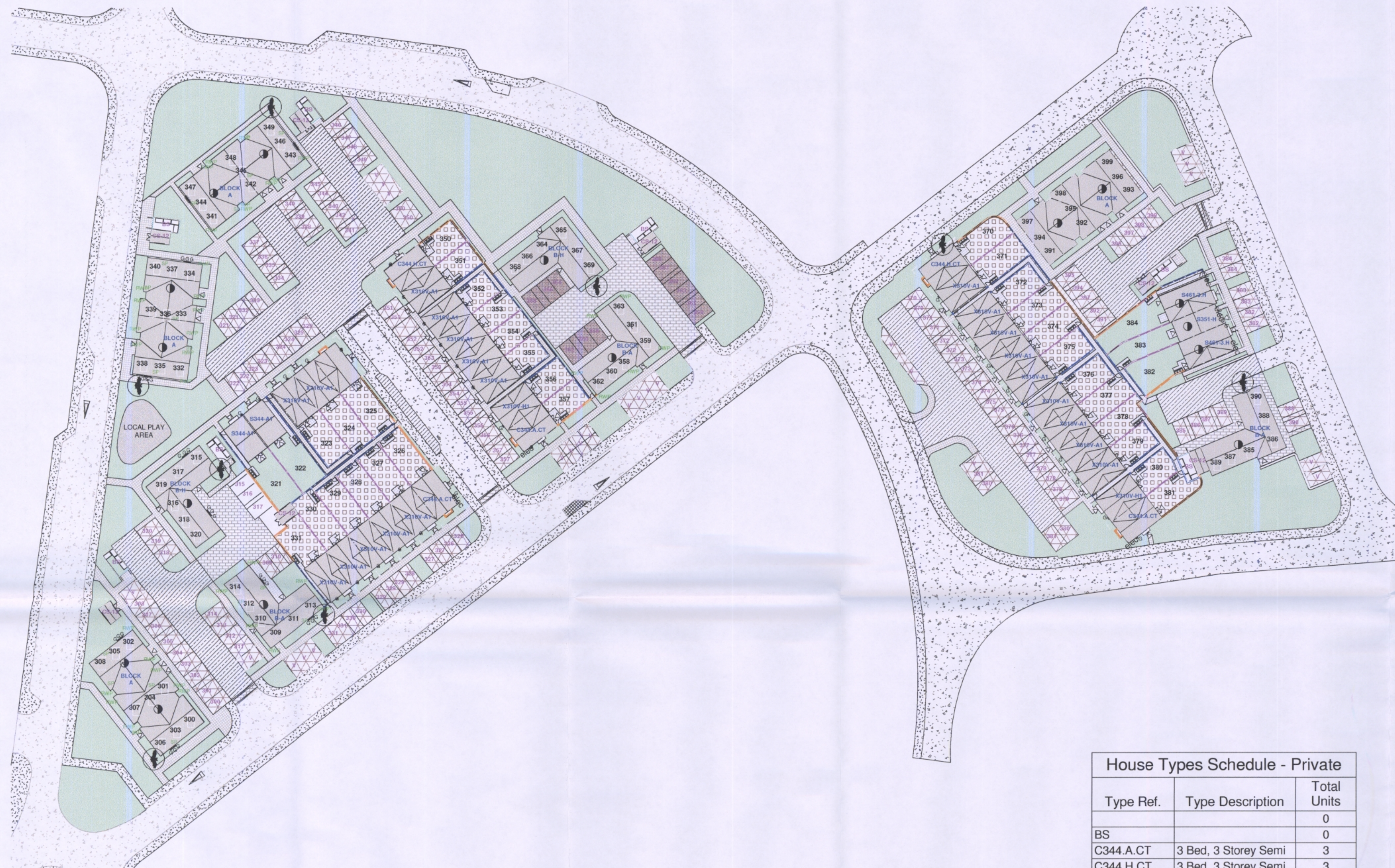
1 Fence Key Plan 1 : 500
