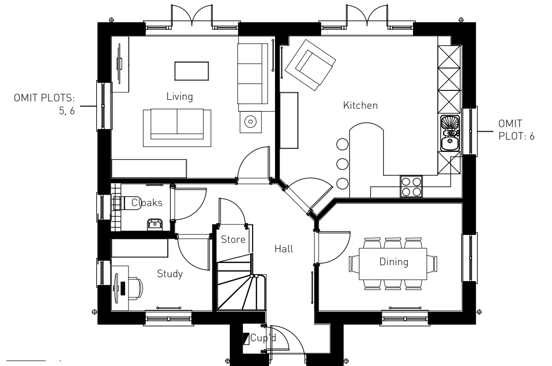
GROUND FLOOR
