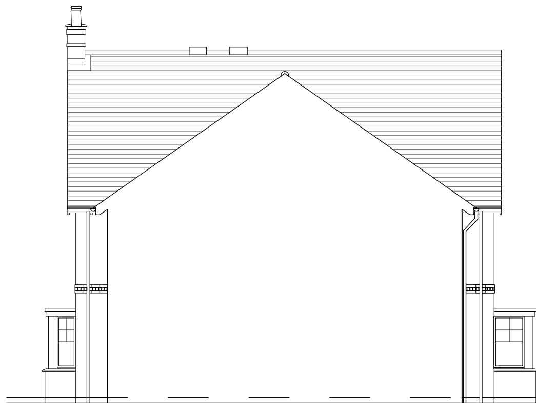
REAR ELEVATION
