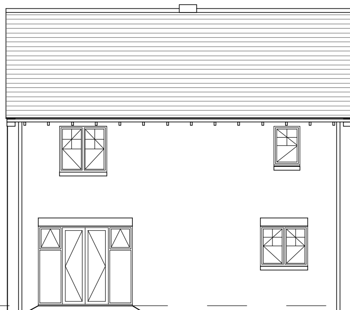
REAR ELEVATION
