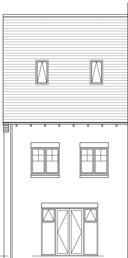
REAR ELEVATION
