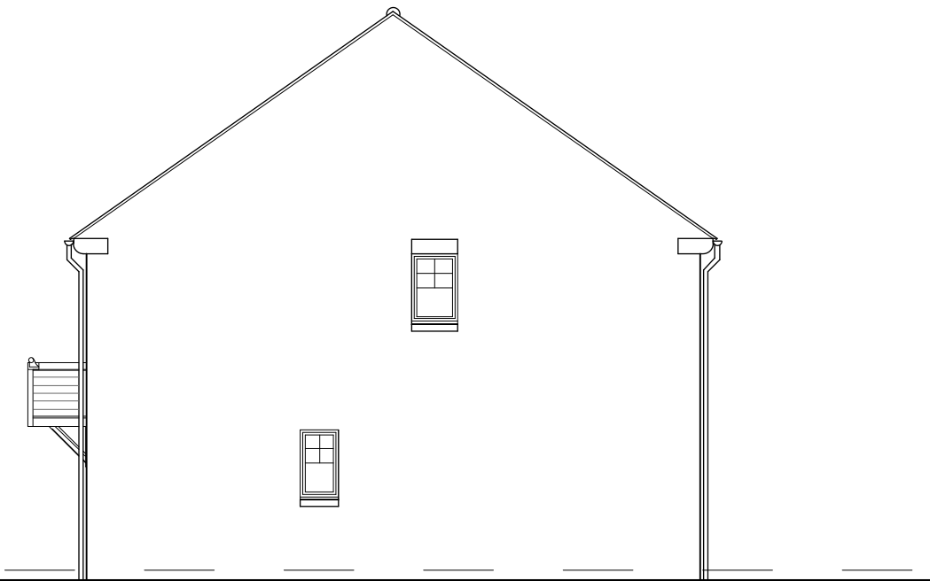
SIDE ELEVATION
