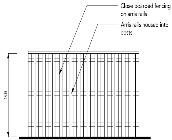
1800mm High Close Board Timber Fence
