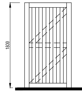
1800mm High Timber Matchboard Access Gate
