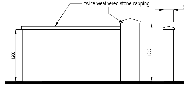
1200mm High Screen Wall with 1350mm High Pier
