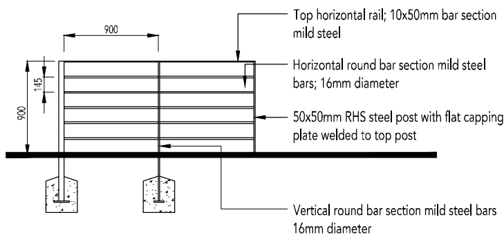
900mm High Metal Estate Railings
