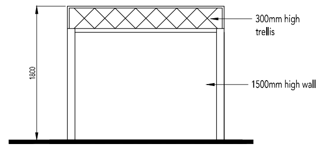
300mm High Trellis on 1500mm High Screen Wall
