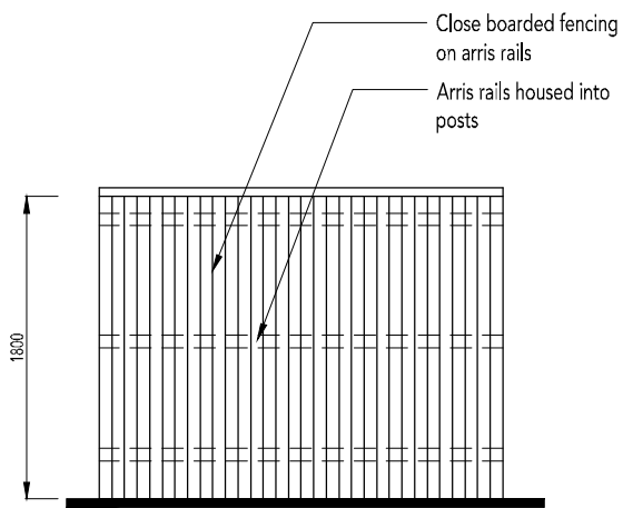
1800mm High Close Board Fence
