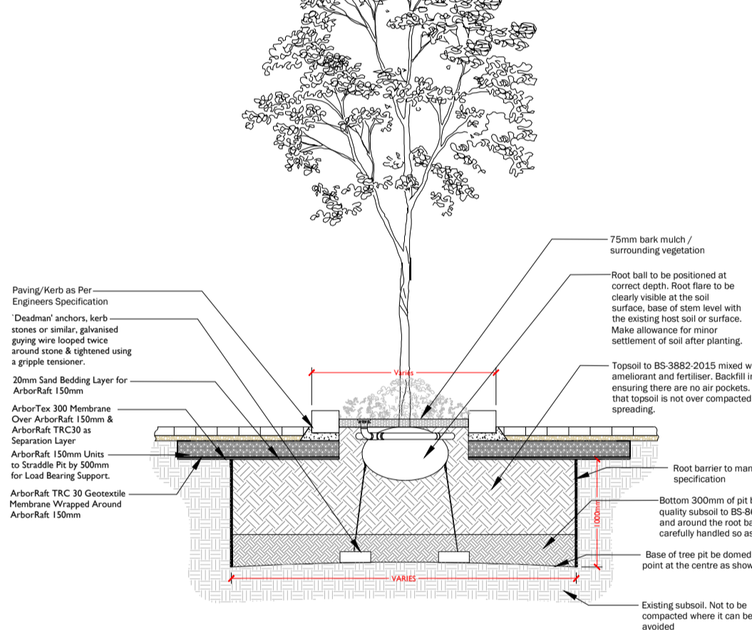
TREE PLANTING IN SMALL AREAS OF SOFT LANDSCAPE DETAIL: 1:50 GREEN-TECH ARBORRAFT SYSTEM
