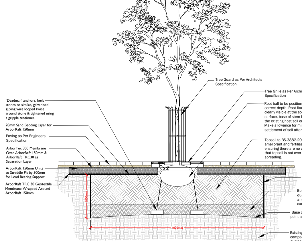
TREE PLANTING IN HARD LANDSCAPE DETAIL: 1:50 GREEN-TECH ARBORRAFT SYSTEM
